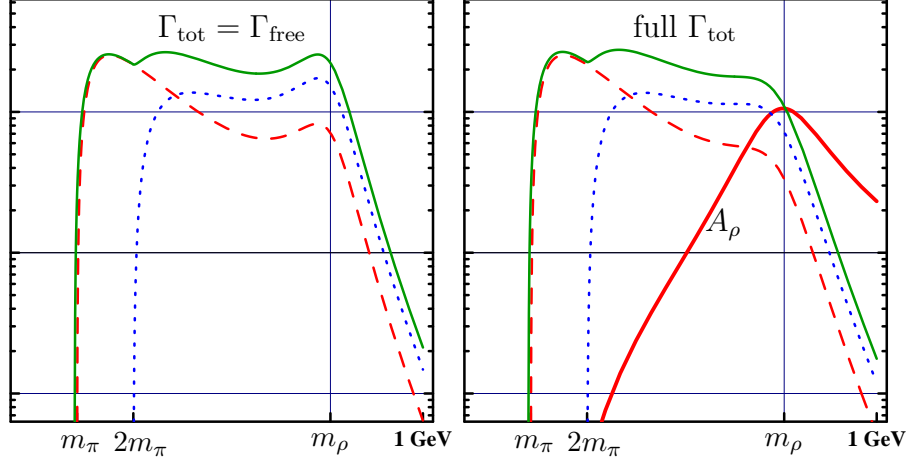
Figure 3: e^+e^- rates (arb. units) as a function of the invariant pair mass m at T = 110 MeV from \pi^+\pi^- annihilation (dotted line) and direct \rho -meson contribution (dashed line), the full line gives the sum of both contributions. Left part: using the free cross section recipe, i.e. with \Gamma_{\text{tot}} = \Gamma_{\rho \pi^+\pi^-} ; right part: the correct partial rates (7). A_\rho is given by the thick line. The calculations are done with \Gamma_{\rho \leftrightarrow \pi\pi}(m_\rho) = 150 MeV and \Gamma_{\rho \leftrightarrow \pi NN^{-1}}(m_\rho) = 70 MeV.
