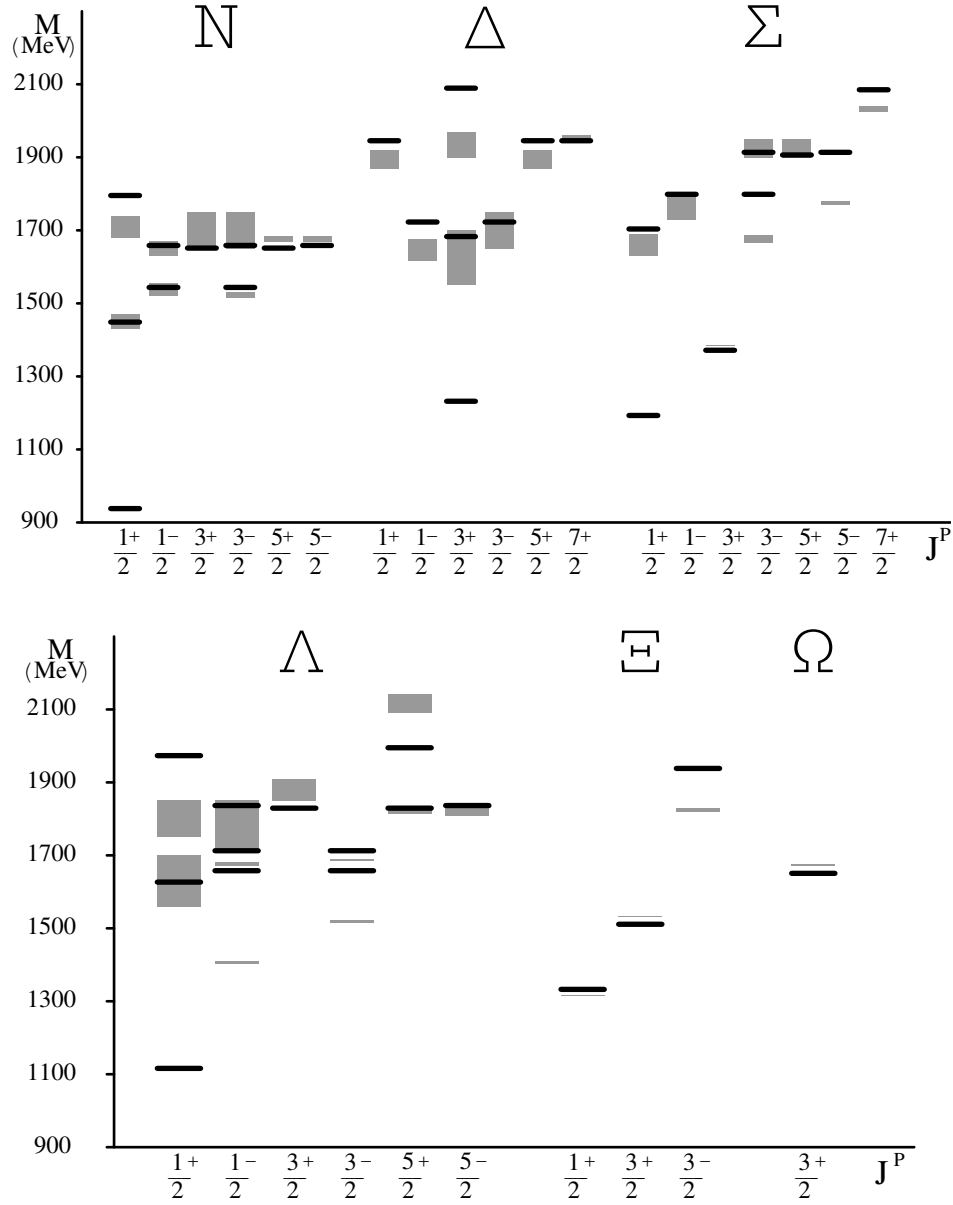
Fig. 1. The energy levels (black lines) for the 3 and 4 star resonances obtained with the Hamiltonian (9) fixing the parameters as described in equation (13). The numerical values of the calculated masses of baryon resonances are reported in Table 2, column M_{calc}^I . The values of the parameters of the Hamiltonian are reported in column (I) of Table 1. The experimental data are taken from PDG [21] (gray boxes).
