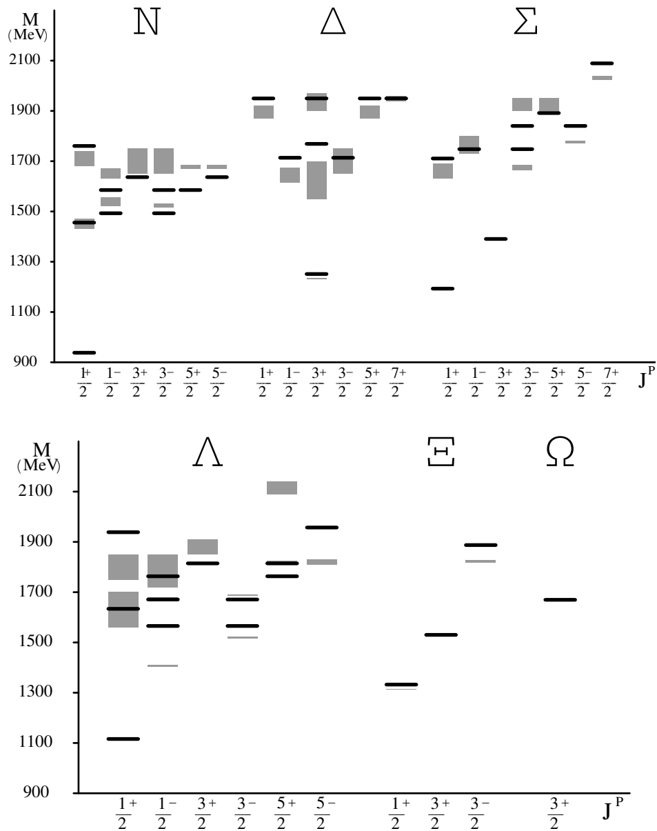
Fig. 2. The energy levels (black lines) for the 3 and 4 star resonances obtained with the Hamiltonian (9) fixing the Hamiltonian parameters by a fitting procedure. The resulting values of the parameters are reported in column II of Table 1, while the numerical values of the calculated masses are also reported in Table 2, column M_{calc}^{II} . The experimental data are taken from PDG [21] (gray boxes).
