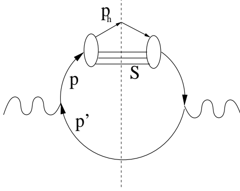
FIG. 1: diagram for single hadron fragmentation in e^+e^- annihilation.
