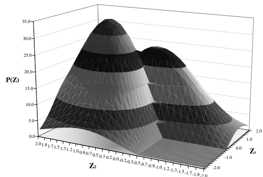
FIG. 4: Optimal sampling distribution, Eq. (9), for the European basket Call option (32) for r = 0.05 , K = 100 , X_1^0 = 100 , X_2^0 = 105 , \sigma_1 = \sigma_2 = 0.3 , T = 1 .
