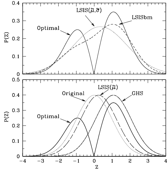
FIG. 3: Sampling probability density functions for a straddle option (30) with r = 0.05 , X_0 = K = 50 , \sigma = 0.3 , T = 1 , as obtained with LSIS [optimizing just the drift, \text{LSIS}(\tilde{\mu}) , both the drift and the volatility, \text{LSIS}(\tilde{\mu}, \tilde{\sigma}) , and using the bi-modal trial density (31), \text{LSISbm} ], and the saddle point approximation (GHS). The original (13) and the optimal (9) sampling densities also shown for comparison.
