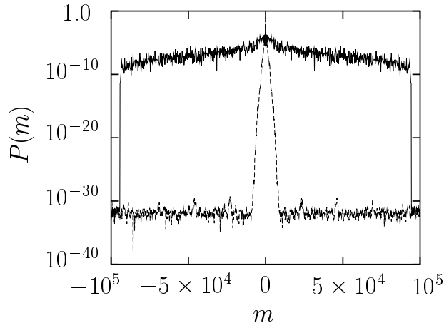
FIG. 3: A comparison between KR (dashed line) and MKR (solid line) in terms of the probability P(m) of finding the system in the state |m\rangle at t = 3000T . \kappa = 3.5 , \tau = 0.1 , and the initial state is |0\rangle . Fluctuations of P(m) below the 10^{-30} level are due to numerical cutoff errors.
