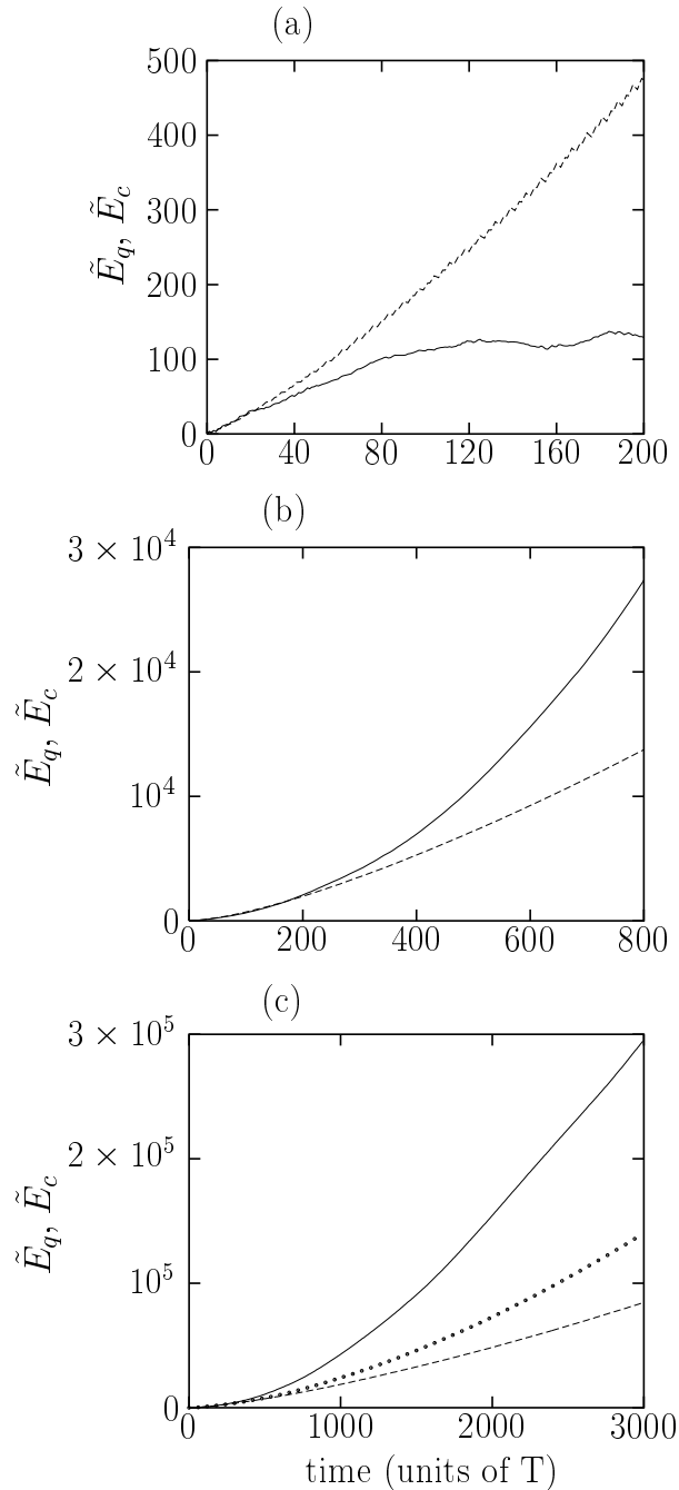
FIG. 2: The time dependence of the average dimensionless scaled rotational energy, denoted \tilde{E}_q and \tilde{E}_c for quantum and classical ensembles, respectively, for (a) KR, (b) MKR, and (c) MKR over even longer time scales, with \kappa = 3.5 . Solid lines denote quantum results for \tau = 0.1 , dashed lines denote classical results. The discrete points in (c) represent quantum results for \tau = 0.01 . Note that in (b) and (c) quantum results are well above the classical results.
