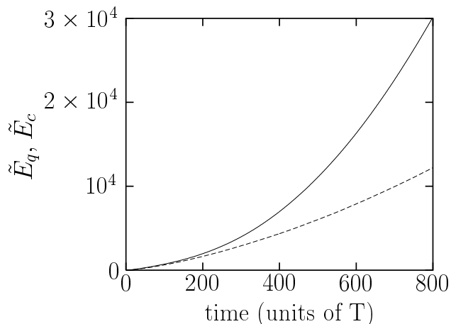
FIG. 4: As in Fig. 2b except that the initial condition, the periodic boundary condition, the values of \tau and \kappa are all changed (see the text for details). The classical initial distribution function is chosen to be identical with the Wigner function of the initial quantum state.
